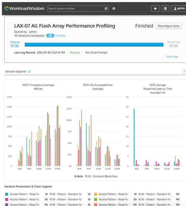
Figure 11: Extract of output report of Workload Iterator function, showing effect of access pattern, block size, queue depth, load throughput, and data reduction ratio on key performance metrics.
